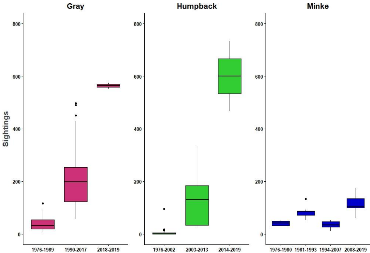
Supplementary Figure S1. Sightings in the Salish Sea Study area (1976-2019) and the results of non-parametric changepoint analysis by species.
