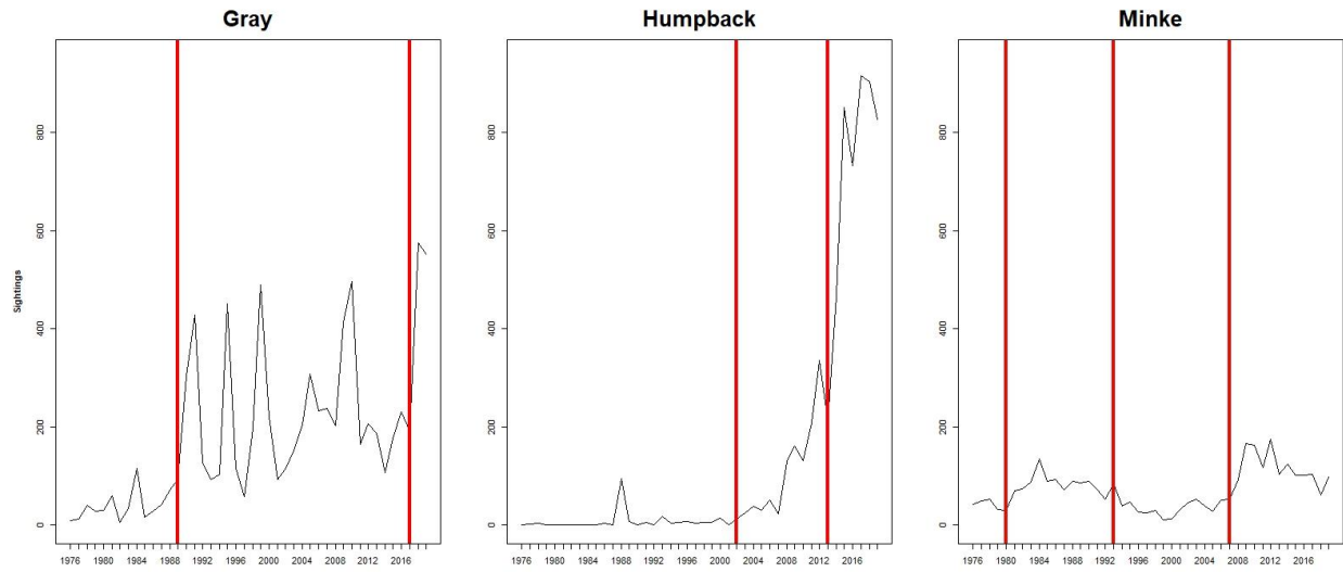
Supplementary Figure S1. Sightings in the Salish Sea Study area (1976-2019) and the results of non-parametric changepoint analysis by species.
