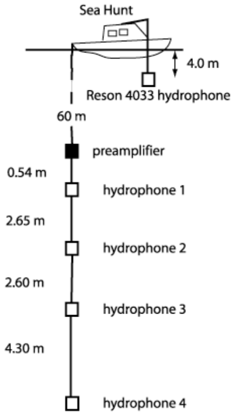
Figure 1. Schematic diagram of the depths of vertical hydrophone array elements and broadband hydrophone (Reson 4033) used in the preparation of this report. All distances are in meters.
