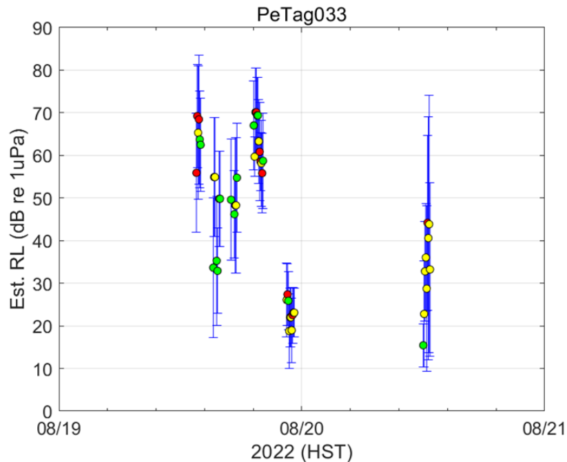
Figure 29 - Median RLs for PeTag033 in stoplight colors (green for few pings during 5-min bin, yellow for moderate number of pings, red for a high number of pings) with error bars giving the ± 2 SD values.
