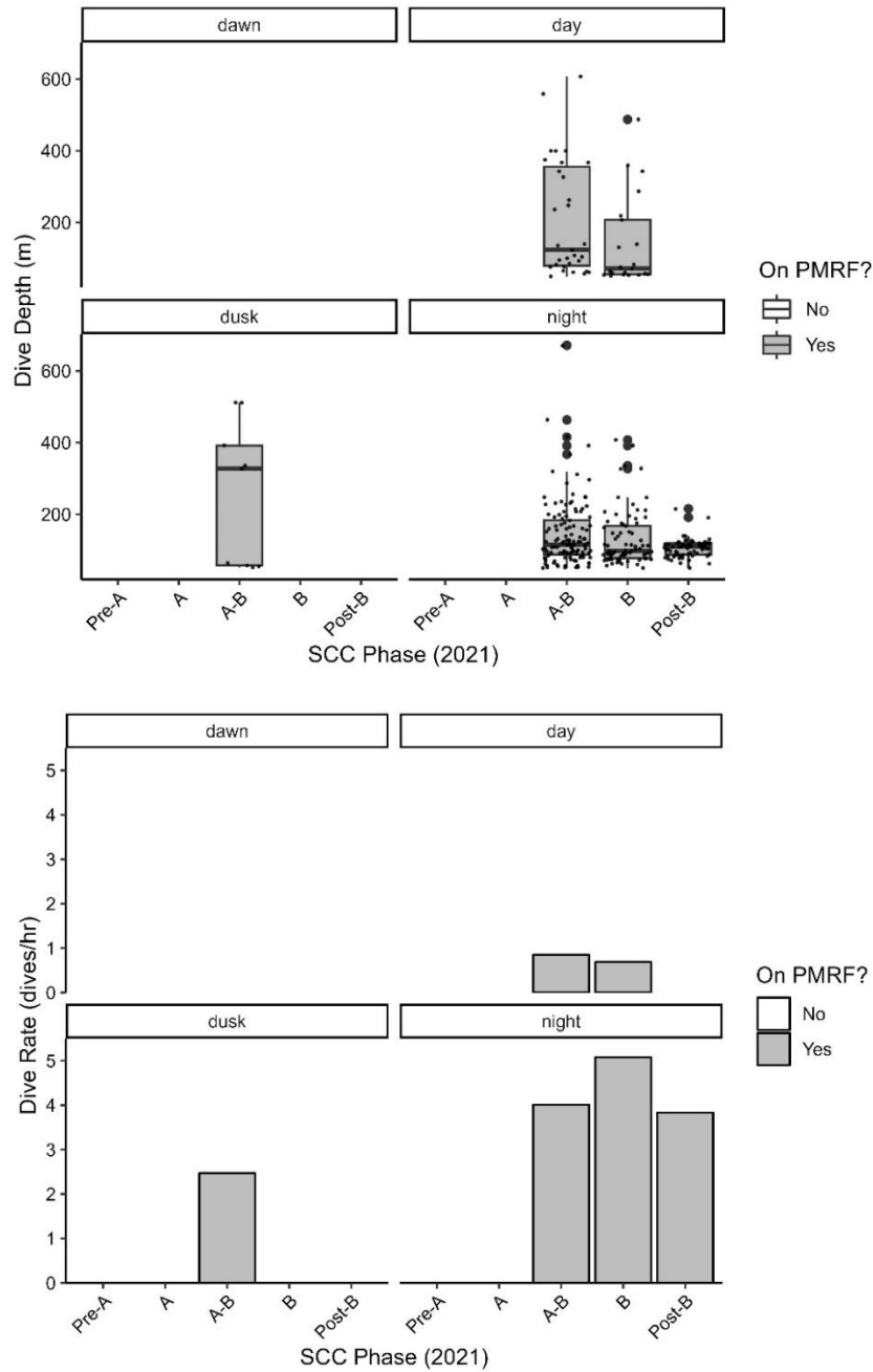
Figure 38 - Top. Boxplot showing dive depths of TtTag039 by SCC Phase and time of day. Bottom. Barplot showing dive rates of TtTag039 by SCC Phase and time of day. Maximum estimated RL from MFAS for this individual was 100.0 dB.
