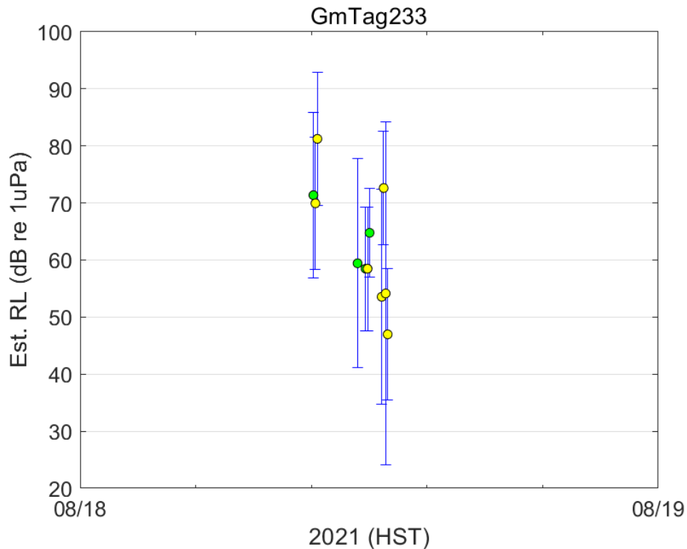
Figure 8 - Median RLs for GmTag233 in stoplight colors (green for few pings during 5 min bin, yellow for moderate number of pings, red for a high number of pings) with error bars giving the \pm 2 SD values.
