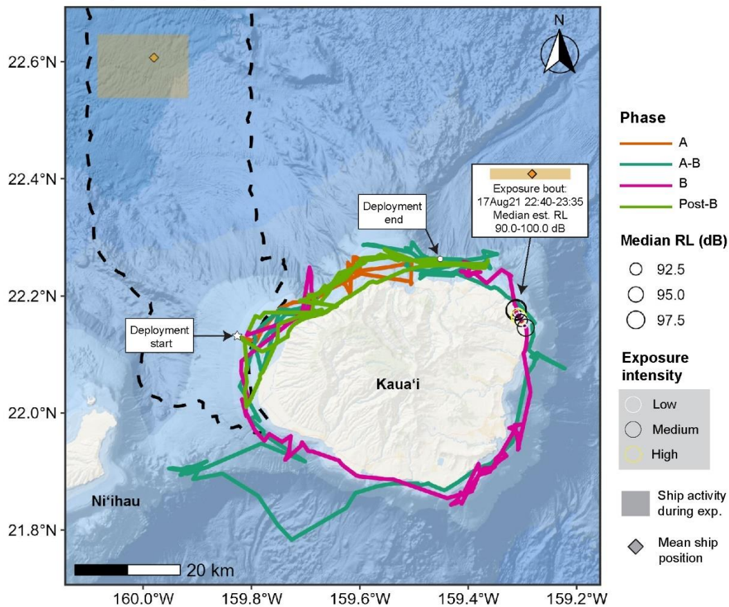
Figure 37 - Movements of TtTag039 during the August 2021 SCC event (see text for description of phases). The maximum, median estimated received levels (RLs) that occurred during each 5-minute exposure bin are plotted as open circles, with the size of the circle scaled to RL level and times given in GMT. Additionally, the RL circles are colored by “intensity” which is characterized by the frequency of MFAS exposures that occurred during that given 5-minute exposure bin. The shaded rectangular polygons represent the area of ship activity during each of the three MFAS bouts that TtTag039 was exposed during and the corresponding diamond points represent the mean ship location during each bout. Note that After is restricted to three days after the end of the SCC. The dashed black line represents the PMRF boundary.
