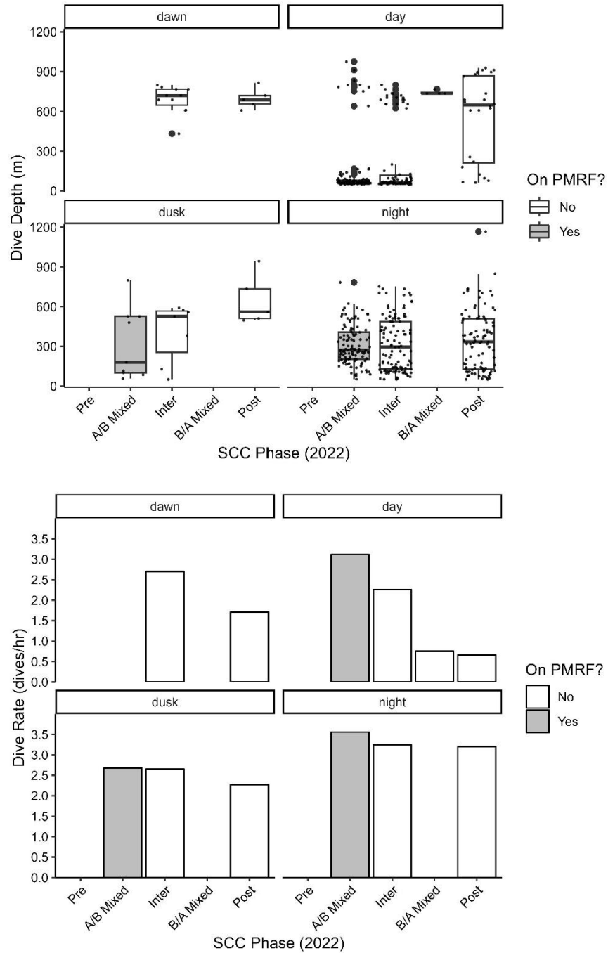
Figure 19 - Top. Boxplot showing dive depths of GmTag237 by SCC Phase and time of day. Bottom. Barplot showing dive rates of GmTag237 by SCC Phase and time of day. Maximum estimated RL from MFAS for this individual was 128.8 dB re 1 \mu Pa.
