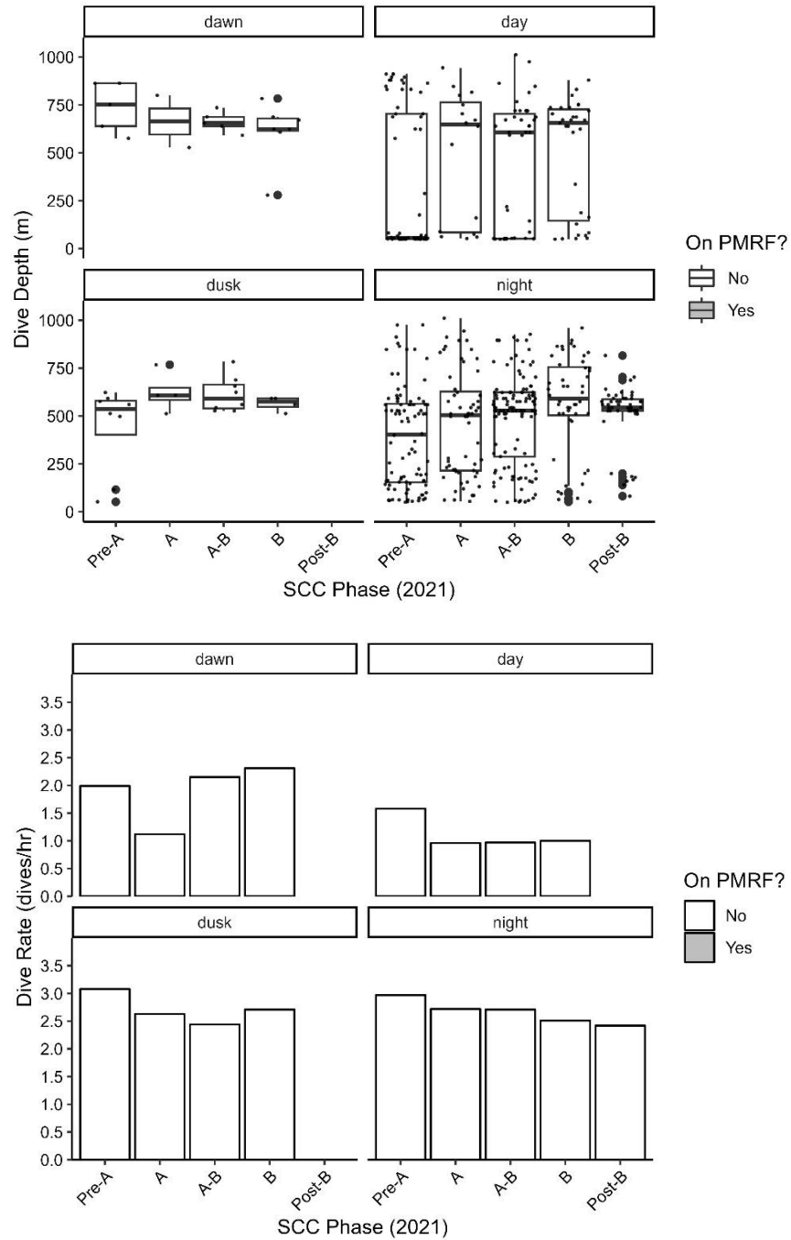
Figure 11 - Top. Boxplot showing dive depths of GmTag232 by SCC Phase and time of day. Bottom. Barplot showing dive rates of GmTag232 by SCC Phase and time of day. Maximum estimated RL from MFAS for this individual was 80.4 dB re 1 \mu Pa.
