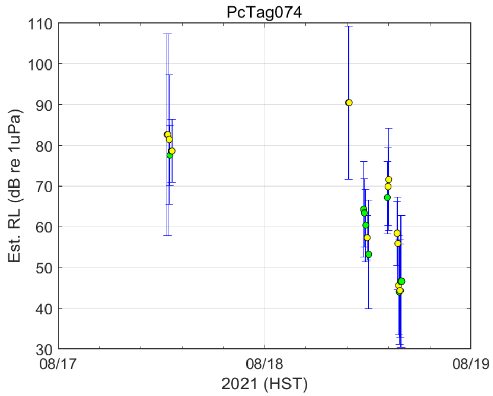
Figure 20 - Median RLs for PcTag074 in stoplight colors (green for few pings during 5-min bin, yellow for moderate number of pings, red for a high number of pings) with error bars giving the \pm 2 SD values.
