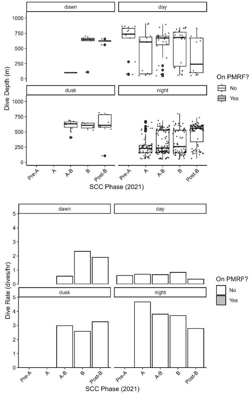
Figure 12 - Top. Boxplot showing dive depths of GmTag233 by SCC Phase and time of day. Bottom. Barplot showing dive rates of GmTag233 by SCC Phase and time of day. Maximum estimated RL from MFAS for this individual was 81.2 dB re 1 \mu Pa.
