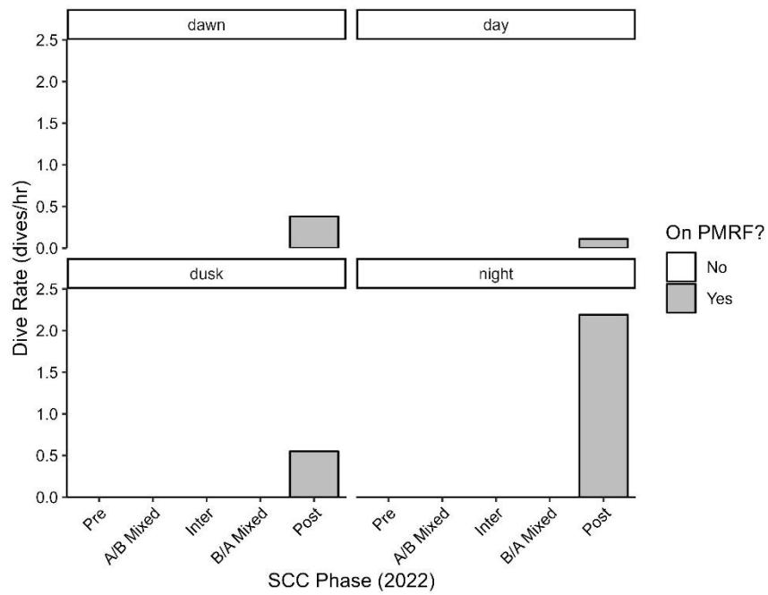
Figure 44 - Top. Boxplot showing dive depths of SbTag025 by SCC Phase and time of day. Bottom. Barplot showing dive rates of SbTag025 by SCC Phase and time of day.
