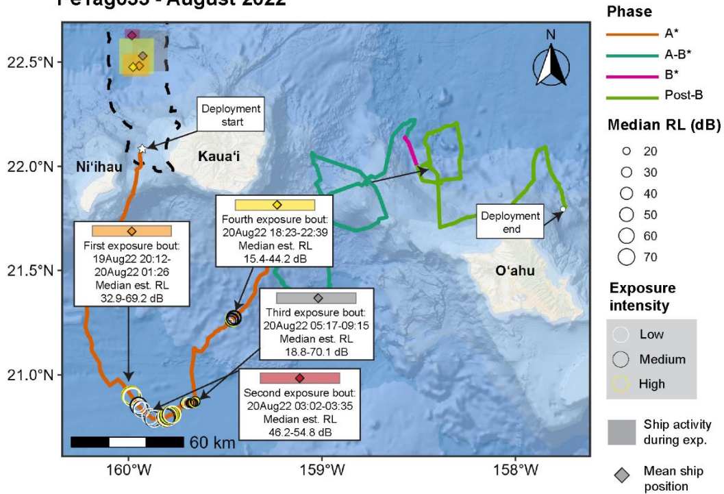
Figure 31 - Movements of PeTag033 during the August 2022 SCC event, including extensive movements away from the range after exposure phases. Note that for this particular event, ship-based MFAS activity occurred during both A and B phases. The maximum, median estimated received levels (RLs) that occurred during each 5-minute exposure bin are plotted as open circles, with the size of the circle scaled to RL level and times given in GMT. Additionally, the RL circles are colored by “intensity” which is characterized by the frequency of MFAS exposures that occurred during that given 5-minute exposure bin. The shaded rectangular polygons represent the area of ship activity during each of the MFAS bouts that PeTag033 was exposed during and the corresponding diamond points represent the mean ship location during each bout. Note that After is restricted to three days after the end of the SCC. The dashed black line represents the PMRF boundary.
