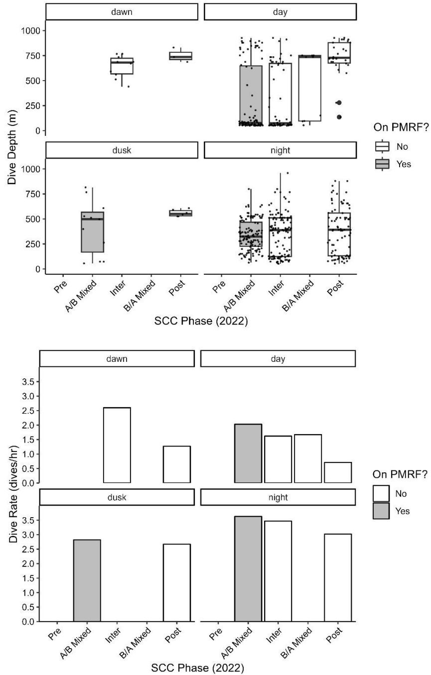
Figure 18 - Top. Boxplot showing dive depths of GmTag235 by SCC Phase and time of day. Bottom. Barplot showing dive rates of GmTag235 by SCC Phase and time of day. Maximum estimated RL from MFAS for this individual was 129.2 dB re 1 \mu Pa.
