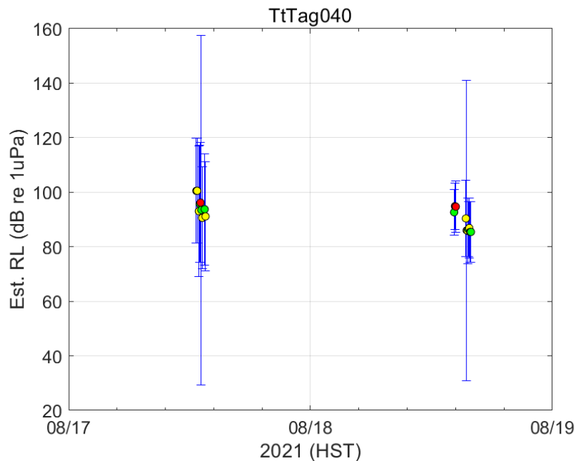
Figure 39 - Median RLs for Tt040 in stoplight colors (green for few pings during 5-min bin, yellow for moderate number of pings, red for a high number of pings) with error bars giving the \pm 2 SD values.
