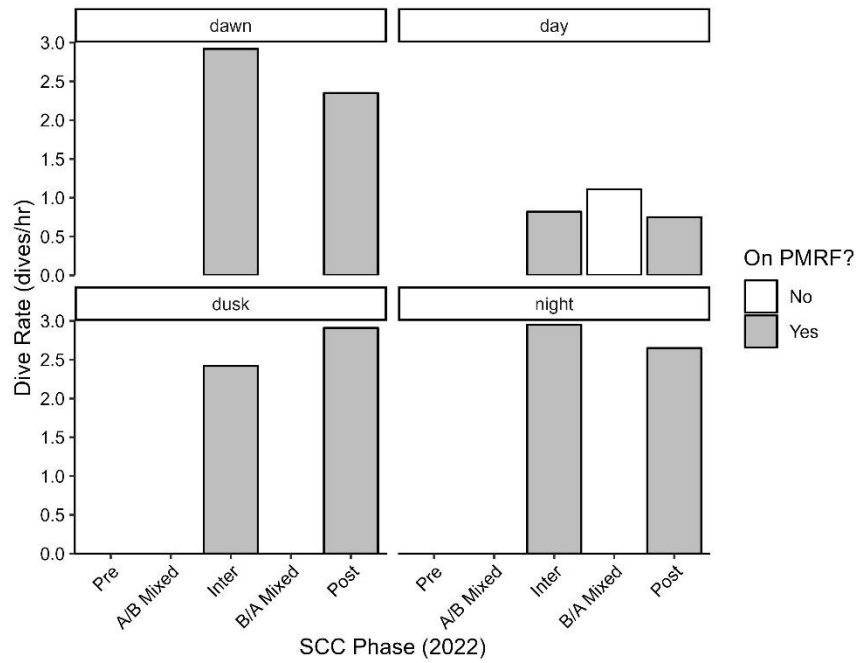
Figure 47 - Top. Boxplot showing dive depths of TtTag041 by SCC Phase and time of day. Bottom. Barplot showing dive rates of TtTag041 by SCC Phase and time of day. Maximum estimated RL from MFAS for this individual was 100.5 dB.
