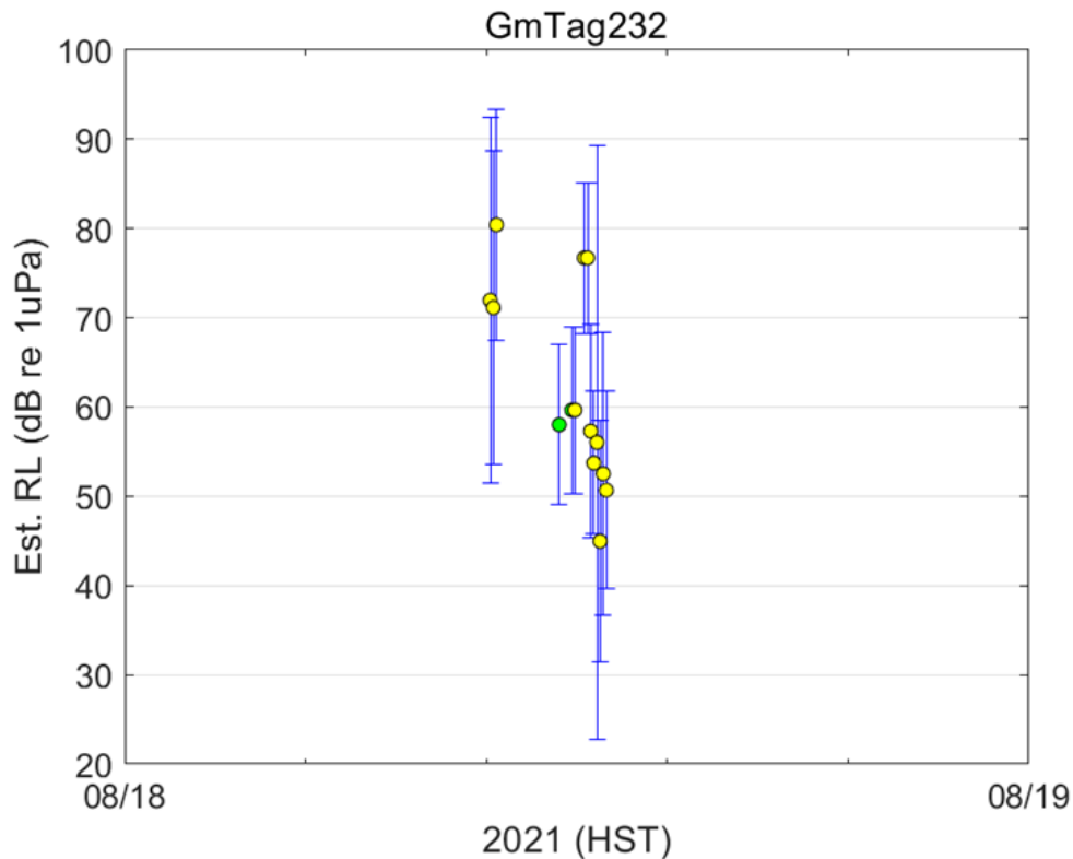
Figure 7 - Median RLs for GmTag232 in stoplight colors (green for few pings during 5 min bin, yellow for moderate number of pings, red for a high number of pings) with error bars giving the \pm 2 SD values.
