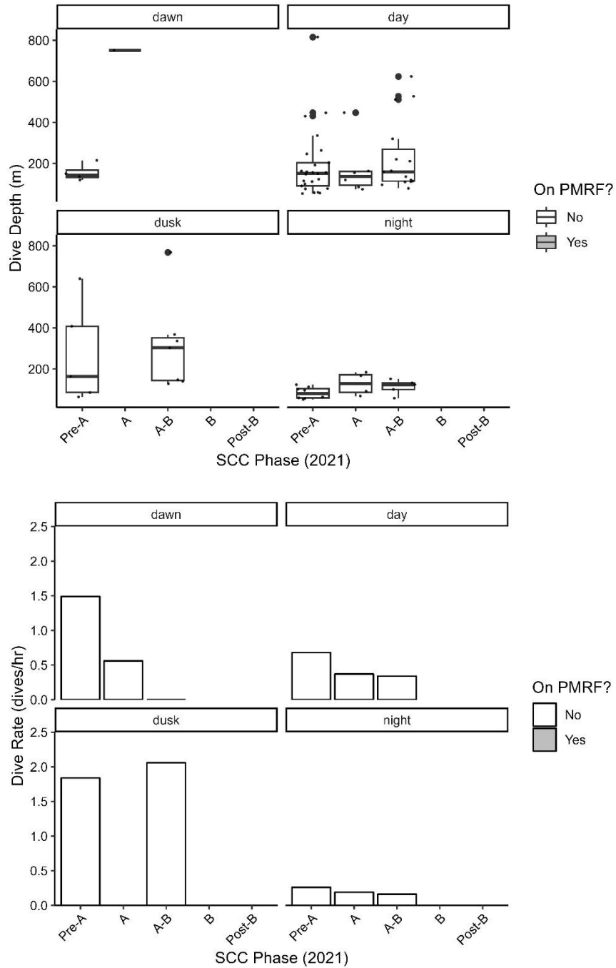
Figure 42 - Top. Boxplot showing dive depths of PcTag074 by SCC Phase and time of day. Bottom. Barplot showing dive rates of PcTag074 by SCC Phase and time of day. Maximum estimated RL from MFAS for this individual was 90.5 dB.
