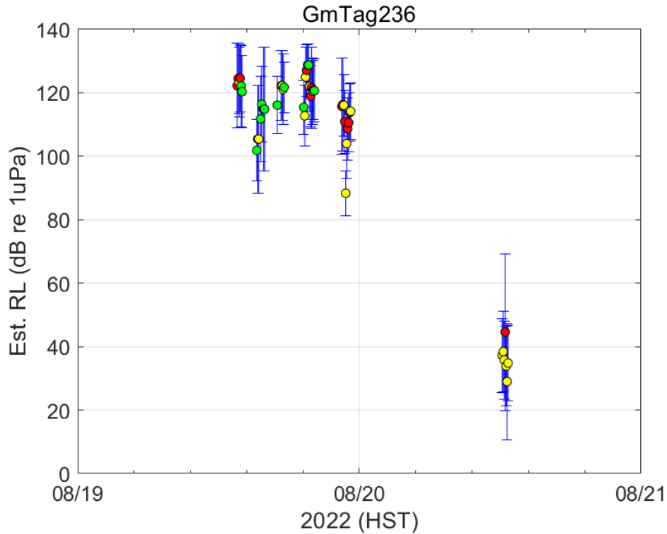
Figure 15 - Median RLs for GmTag236 in stoplight colors (green for few pings during 5 min bin, yellow for moderate number of pings, red for a high number of pings) with error bars giving the \pm 2 SD values.
