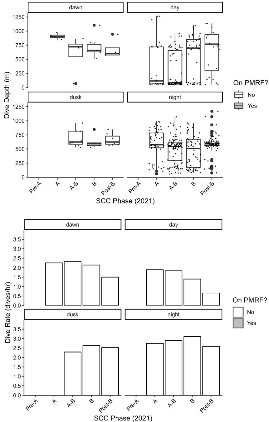
Figure 13 - Top. Boxplot showing dive depths of GmTag234 by SCC Phase and time of day. Bottom. Barplot showing dive rates of GmTag234 by SCC Phase and time of day. Maximum estimated RL from MFAS for this individual was 72.6 dB re 1 \mu Pa.
