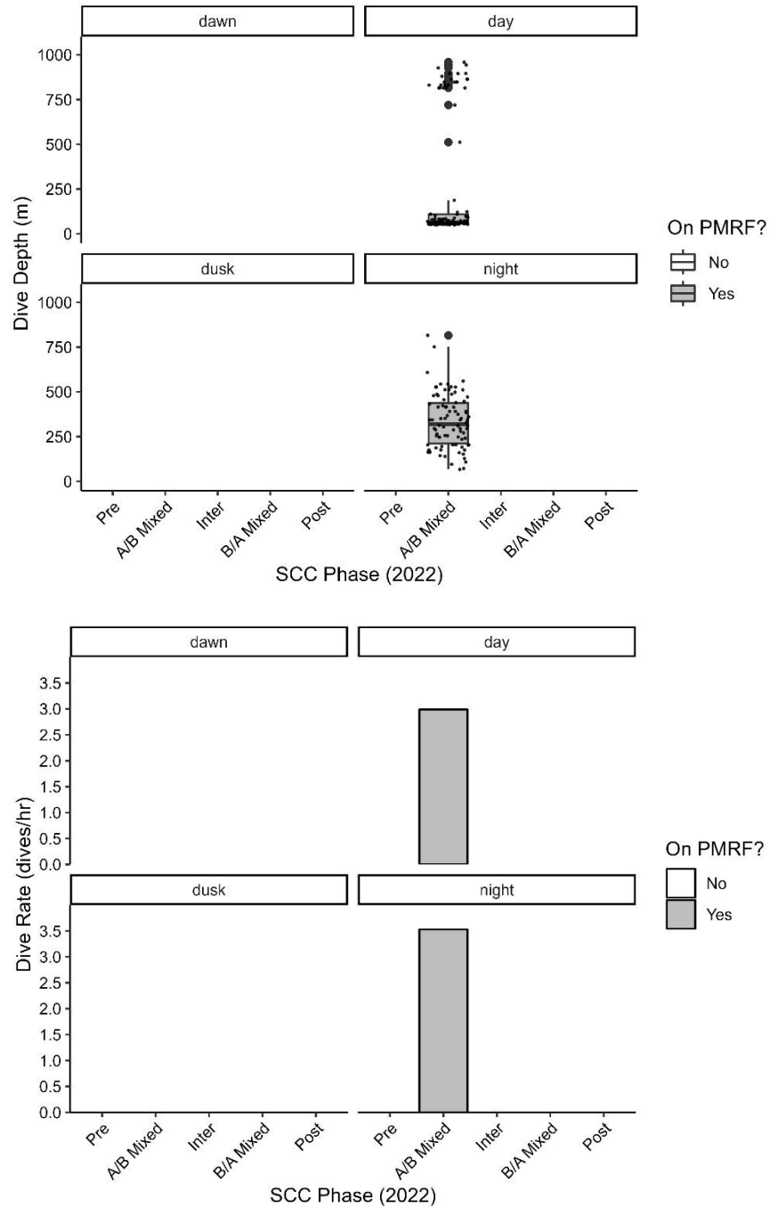
Figure 41 - Top. Boxplot showing dive depths of GmTag236 by SCC Phase and time of day. Bottom. Barplot showing dive rates of GmTag236 by SCC Phase and time of day. Maximum estimated RL from MFAS for this individual was 128.8 dB.
