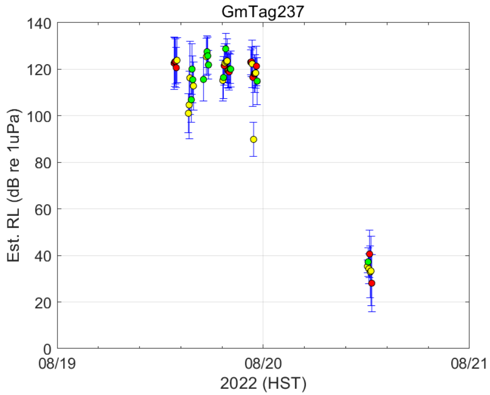
Figure 16 - Median RLs for GmTag237 in stoplight colors (green for few pings during 5 min bin, yellow for moderate number of pings, red for a high number of pings) with error bars giving the \pm 2 SD values.
