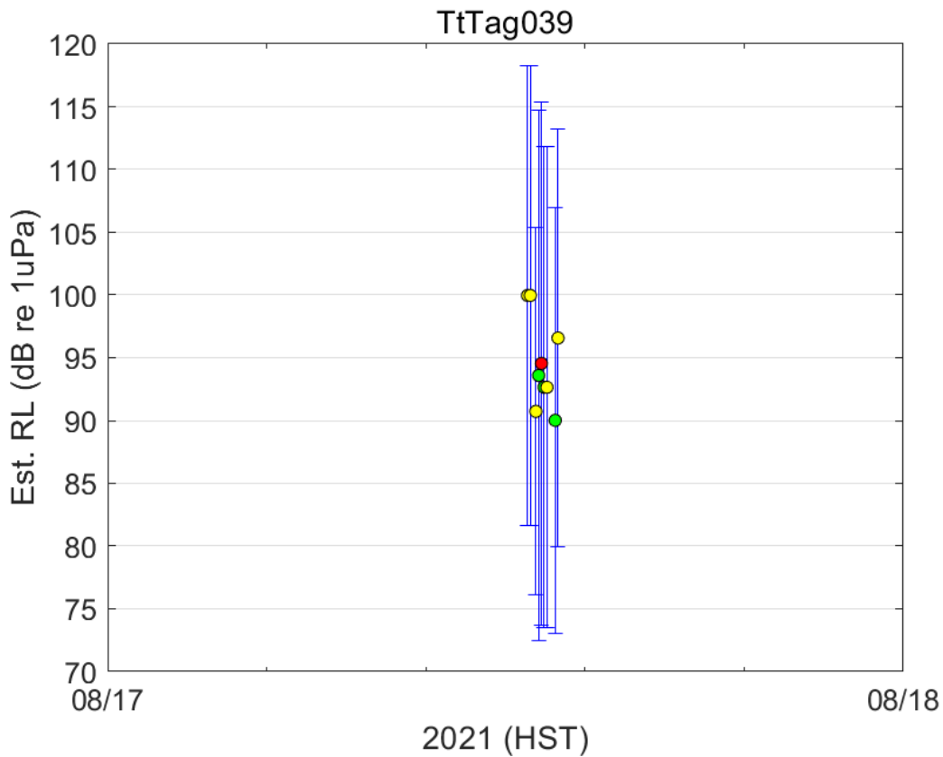
Figure 36 - Median RLs for TtTag039 in stoplight colors (green for few pings during 5-min bin, yellow for moderate number of pings, red for a high number of pings) with error bars giving the \pm 2 SD values.
