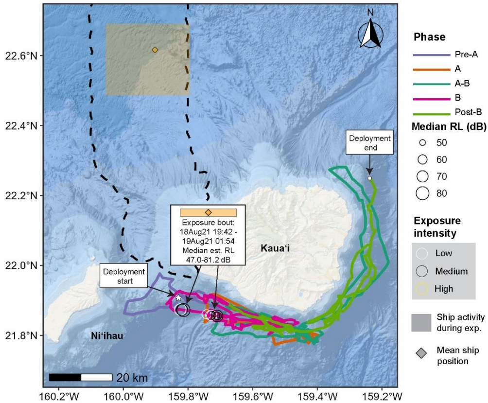
Figure 10 - Movements of GmTag233 during the August 2021 SCC event (see text for description of phases). The maximum, median estimated received levels (RLs) that occurred during each 5-minute exposure bin are plotted as open circles, with the size of the circle scaled to RL level, and time is given in GMT. Additionally, the RL circles are colored by “intensity” which is characterized by the frequency of MFAS exposures that occurred during that given 5-minute exposure bin. The shaded rectangular polygon represents the area of ship activity during each of the three MFAS bouts that GmTag233 was exposed to and the corresponding diamond point represents the mean ship location during the bouts. Note that After is restricted to three days after the end of the SCC. The dashed black line represents the PMRF boundary.
