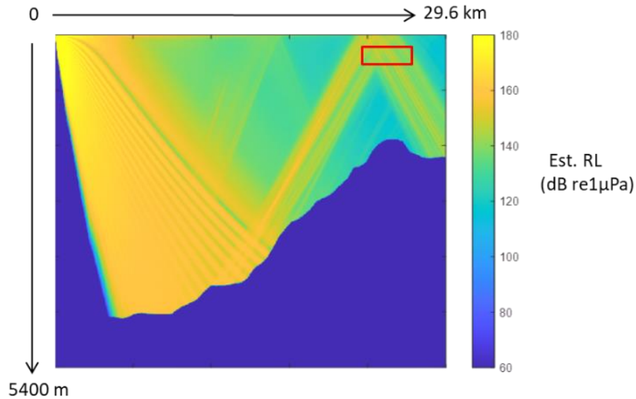
Figure 3 – Example of single slice from ship MFAS source full depth maximum distance estimated receive level in units of dB re 1\mu\text{Pa} . Dark color indicates the seafloor, highlighting the steep angle limitation close to source. The red insert box illustrates potential location in this slice of the animal location using the 95% CI ellipse and depth information.
