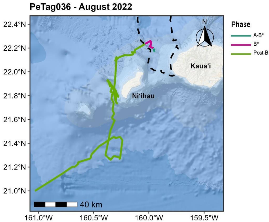
Figure 43 - Top. Map showing crawl model trackline of PeTag035 during the 2022 August SCC. Bottom. Map showing crawl model trackline of PeTag036 during the 2022 August SCC.
