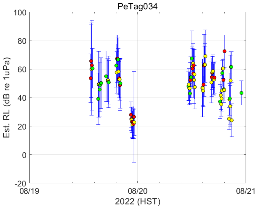
Figure 30 - Median RLs for PeTag034 in stoplight colors (green for few pings during 5-min bin, yellow for moderate number of pings, red for a high number of pings) with error bars giving the \pm 2 SD values.
