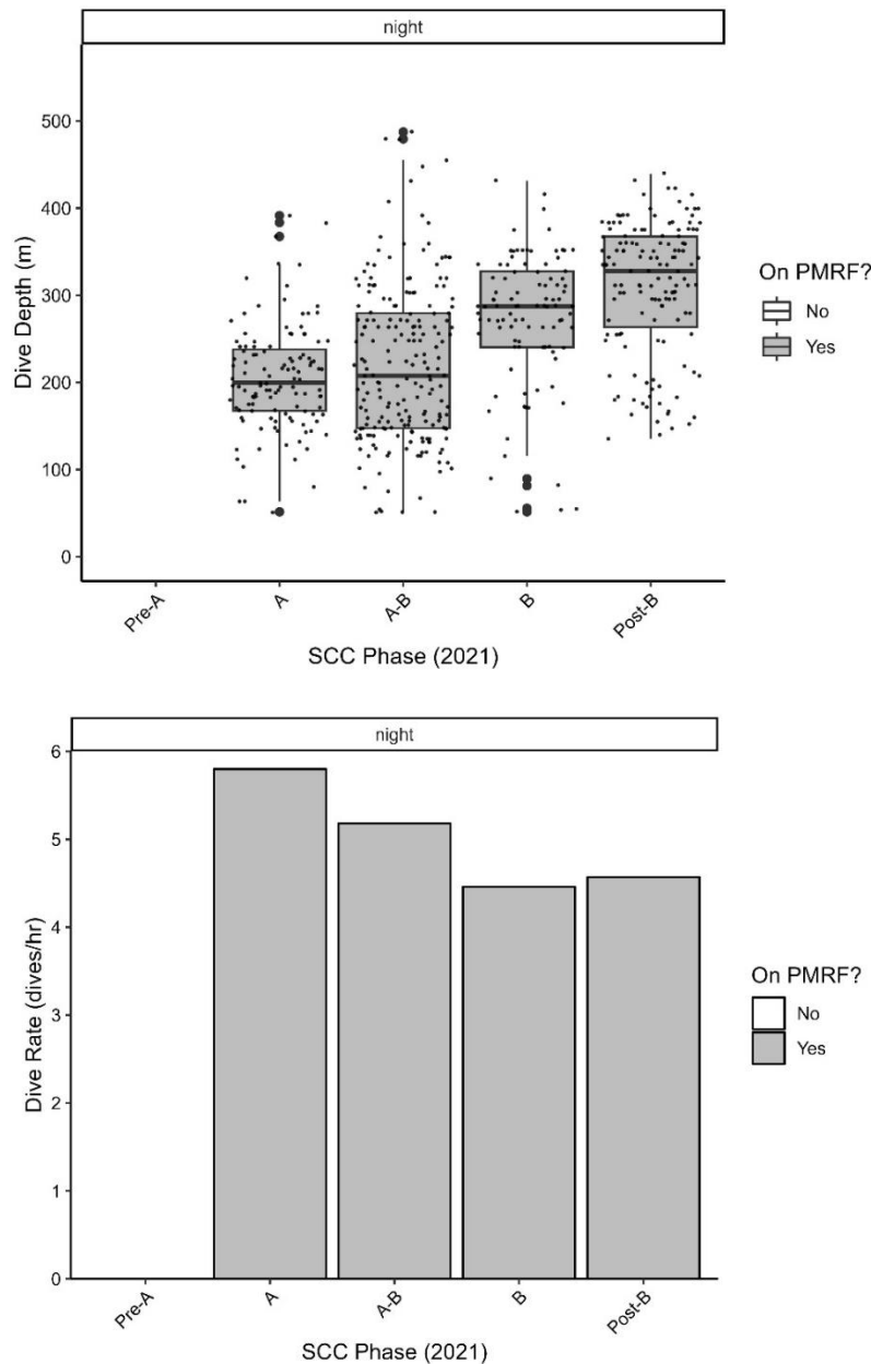
Figure 28 - Top. Boxplot showing dive depths of PeTag031 by SCC Phase and time of day. Bottom. Barplot showing dive rates of PeTag031 by SCC Phase and time of day. Maximum estimated RL from MFAS for this individual was 136.6 dB.
