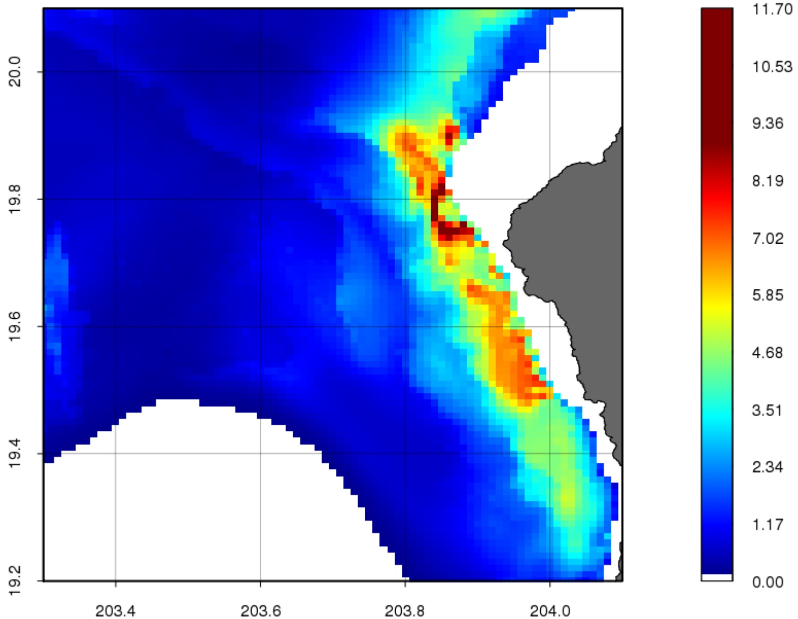
Pilot whales - 2011 - predicted density based on GAMM Z2 \sim s(\text{bathy}) + s(\text{Temp 500m}) + s(\text{W200})
